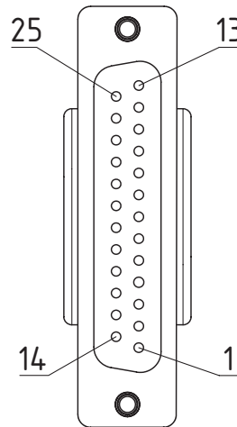
C5: D-SUB 25 (female)
