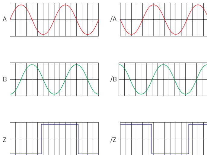
Z Length depend on magnetic pole length
